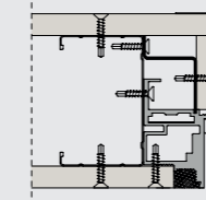
Gipskarton Plasterboard
